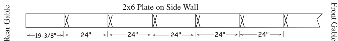
Detail 'A'
